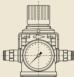
Pressure reducing valve (kit)
