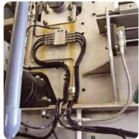
In this corrosive environment, a stainless steel Lincoln Quickclub system is lubricating and purging 32 points on a belt press in a wastewater plant.
