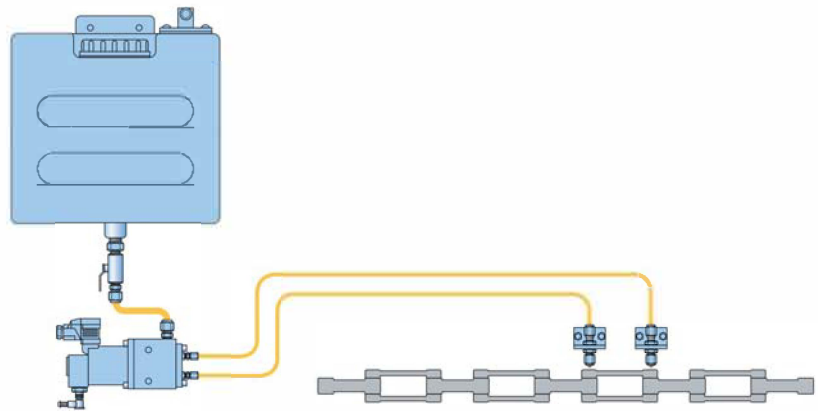
PMA metered squirt system No air required
