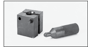
Fig. R58 — Vise Block with Flaring Pin
