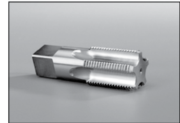
Fig. R78 — BSPP Straight Thread Tapping Tool
