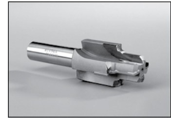
Fig. R82 — ISO 6149-1 Straight Thread Port Counterboring Tool — Small Spotface
