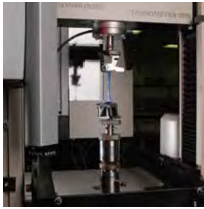
Tensometer
