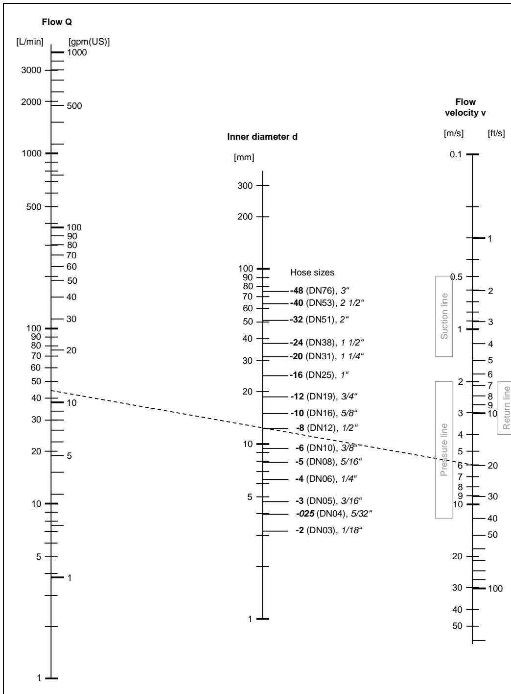
Flow capacity nomogram for the graphic determination of the inner diameter of hydraulic lines
